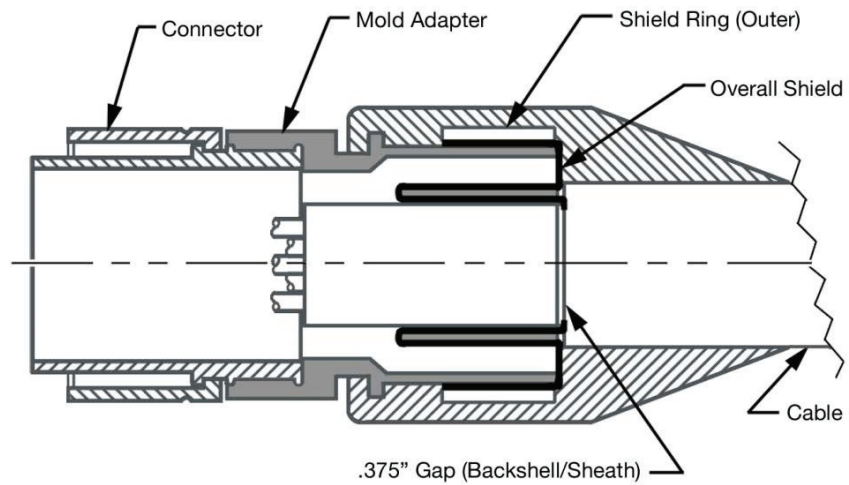
Figure 11. 360-Degree Overall Shield Termination Using a Mold Adapter
