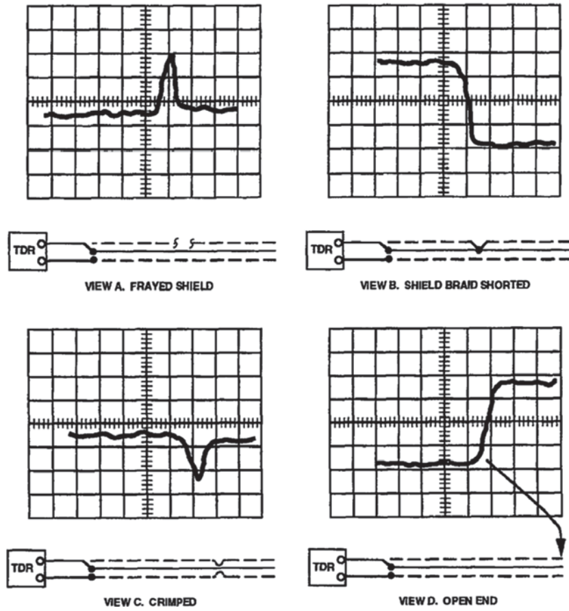
Figure 23. TDR Traces for Coaxial Cable
