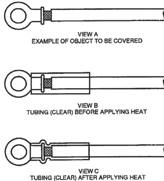
Figure 18. Application of Heat-Reactive Tubing
