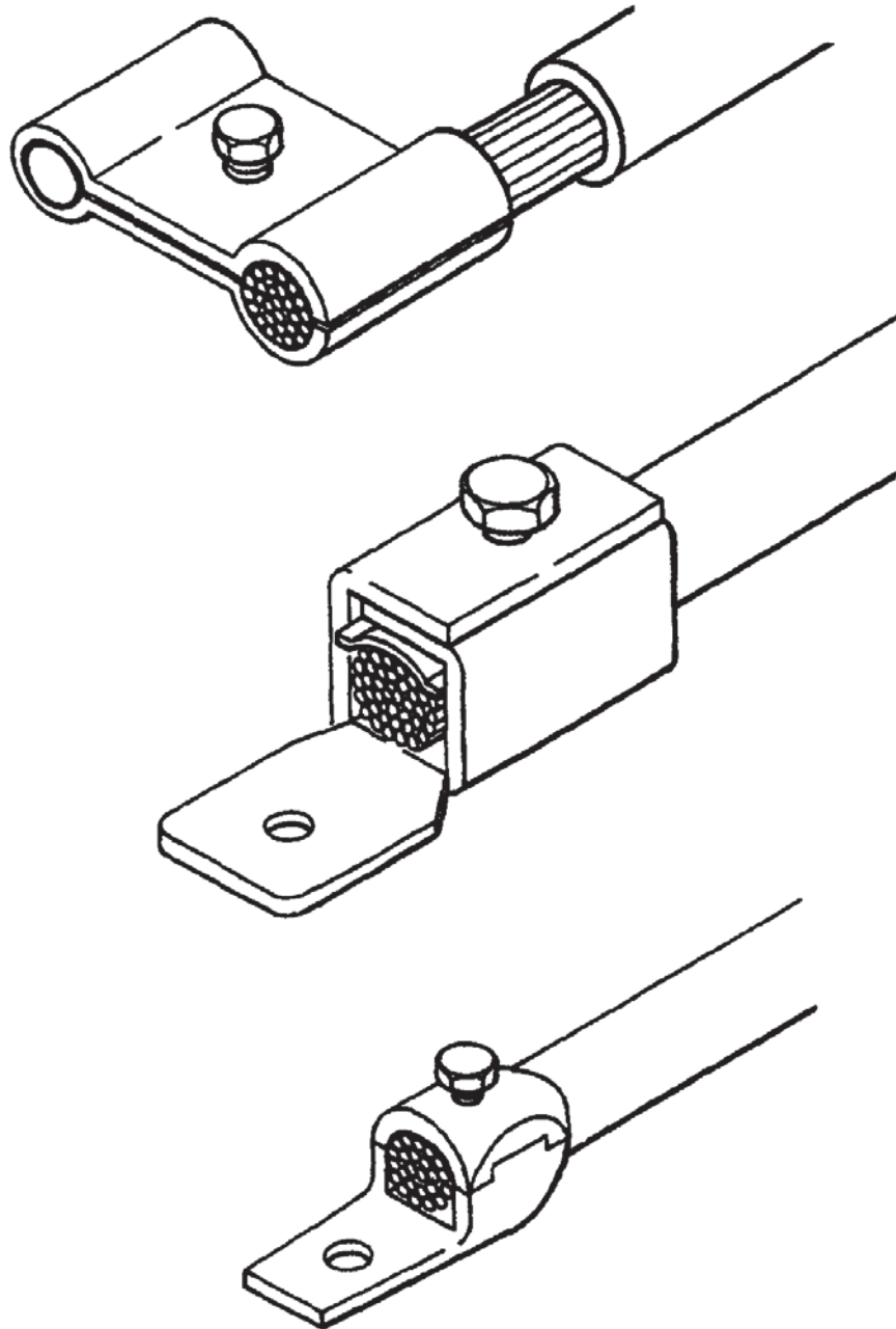
Figure 17. Clamp and Screw End Terminations
