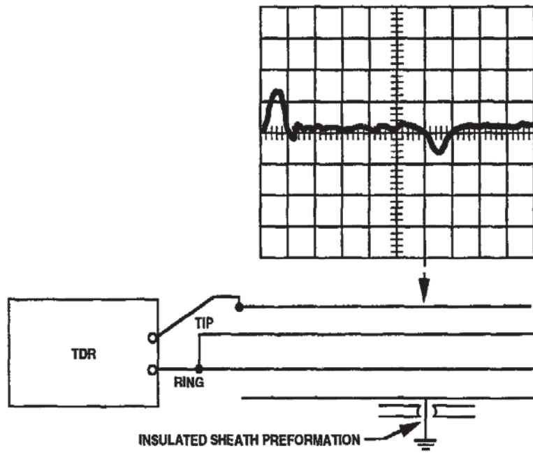
VIEW C. GROUNDED SHEATH FAULT
