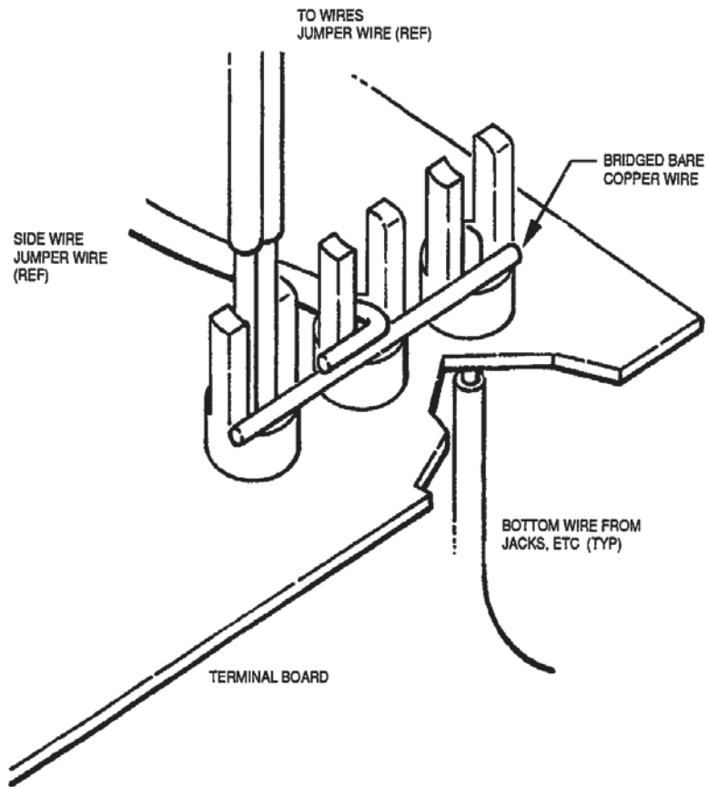
Figure 15. Bridge Bus Terminals
