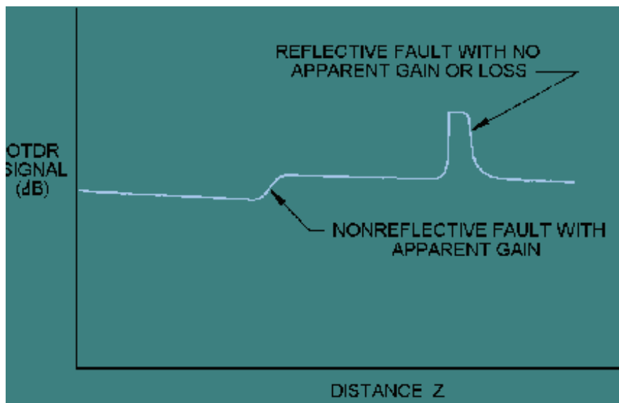
Figure 28. OTDR Trace Showing a Nonreflective Fault With Apparent Gain and a Reflective Fault With No Apparent Loss or Gain
