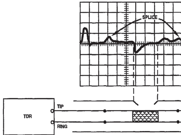
VIEW D. WATER OR MOISTURE FAULT
