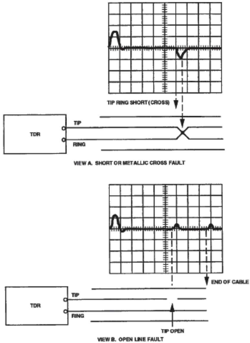
Figure 24. TDR Fault Traces for Twin-Axial Cable (Sheet 1 of 2)
