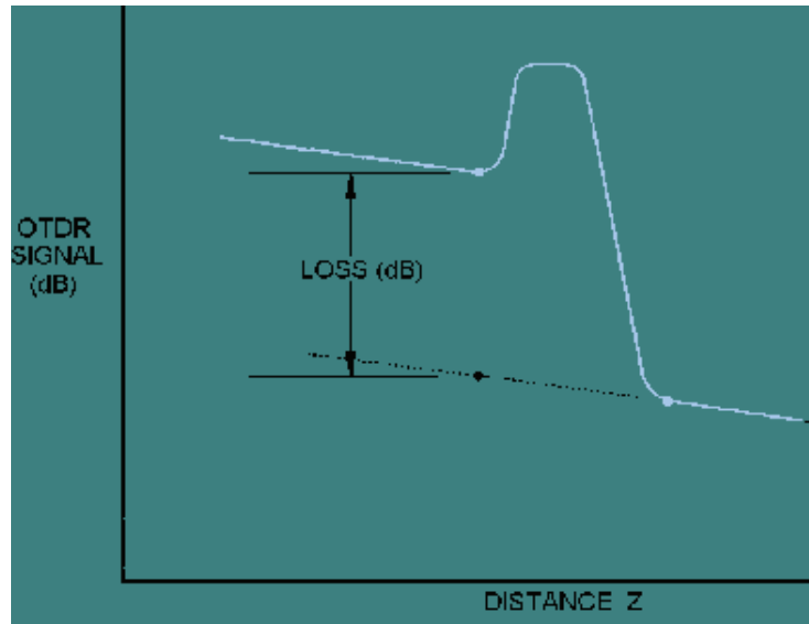
Figure 30. Exaggerated Loss Obtained at Point Defects Exhibiting Gain in One Direction by Conducting the OTDR Measurement in the Opposite Direction
