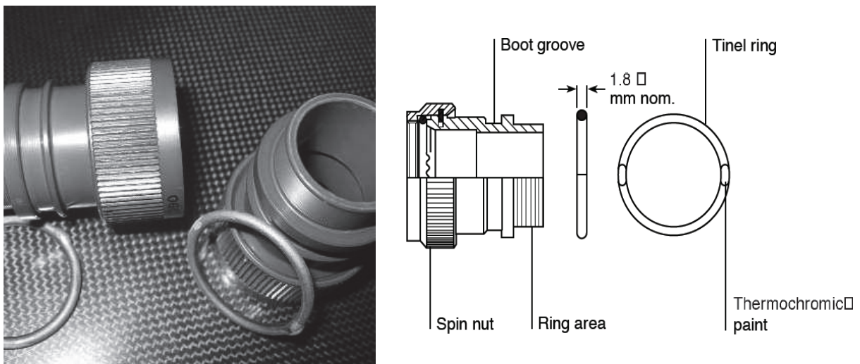
Figure 12. Tinel-Lock Rings and an Example of One Type of Adapter
