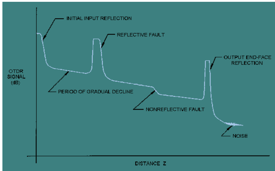
Figure 26. OTDR Trace of an Installed Cable Plant
