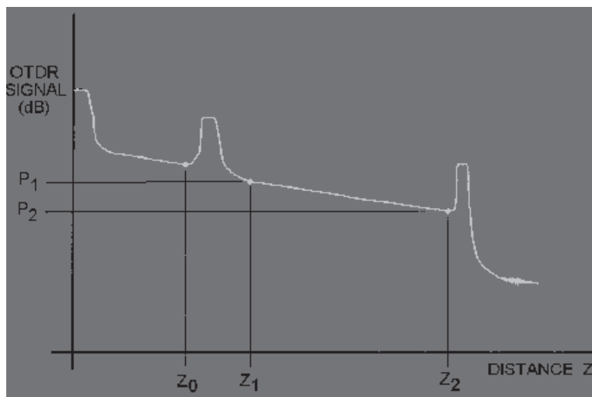
Figure 27. OTDR Measurement Points for Measuring Fiber Attenuation, Using Dead-Zone Fiber
