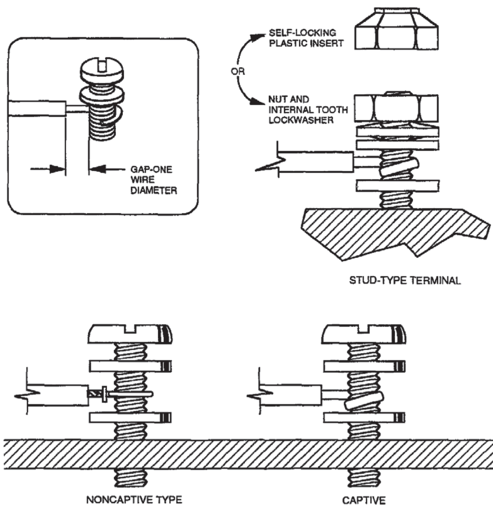
Figure 16. Captive and Noncaptive Nut and Screw Head Terminations
