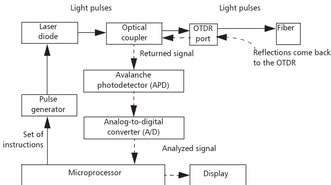
Figure 25. Typical OTDR Block Diagram
