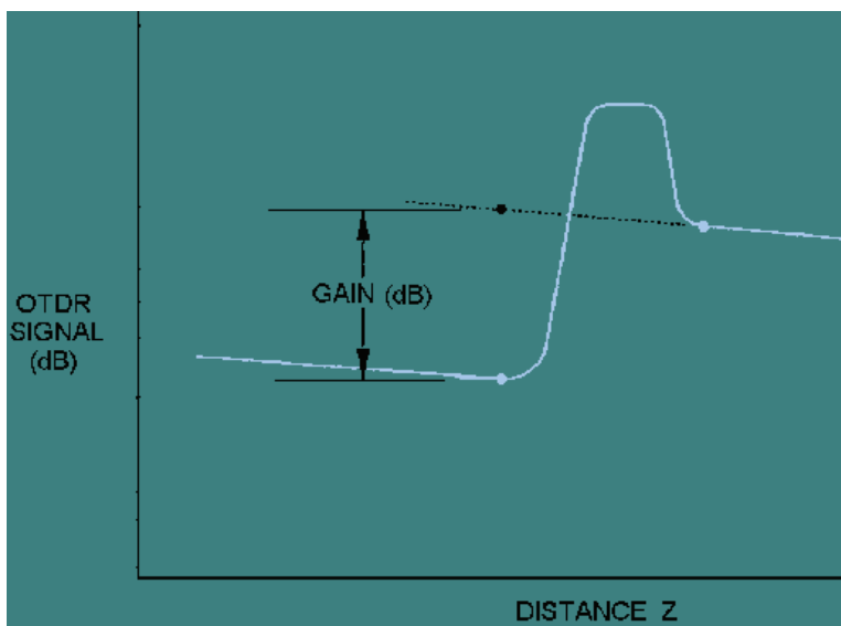
Figure 29. Extrapolation for a Point Defect Showing an Apparent Signal Gain
