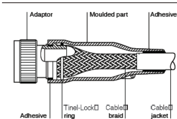
Figure 14. Typical Installation of Tinel-Lock Ring
