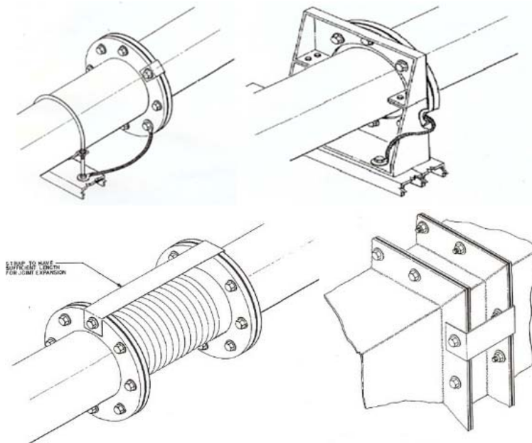
Figure 6. Typical Methods of Providing Electrical Continuity across Mechanical Joints with Different Conductive Material, such as Aluminum to Steel
