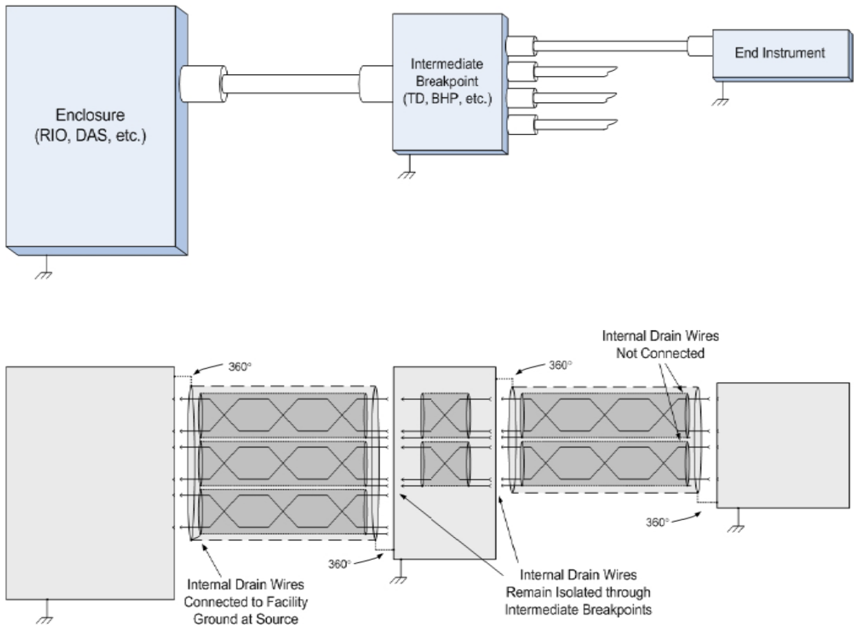
Figure 5. Recommended Shield Terminations
