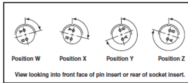
Figure 10. AS50151 Alternate Insert Positions
