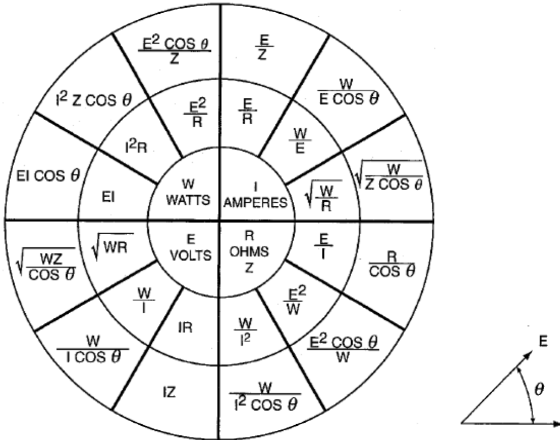
Figure 11. Ohm's Law
