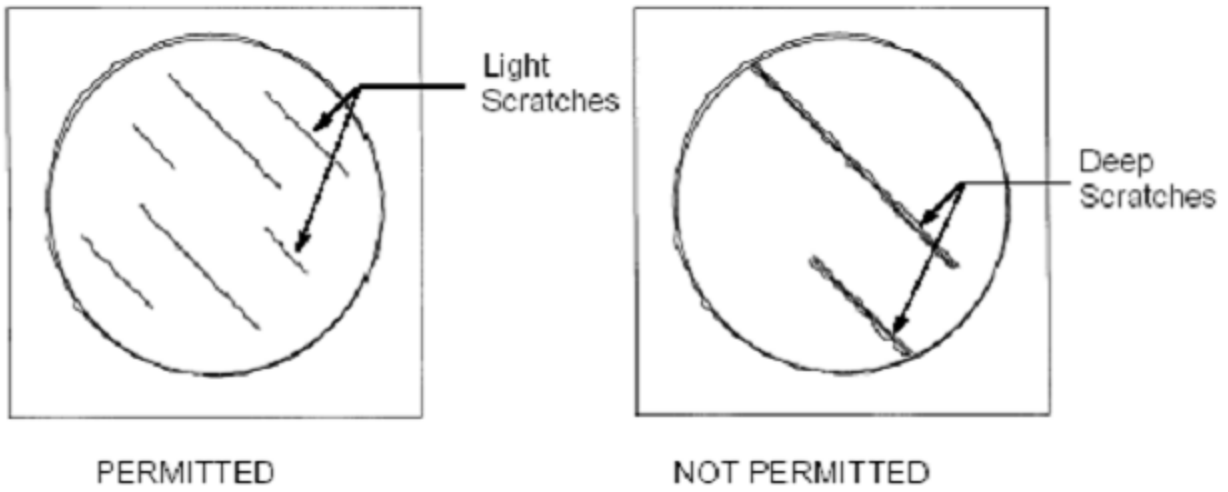
Figure 18. Examples of Scratches on the Endface of an Optical Fiber
