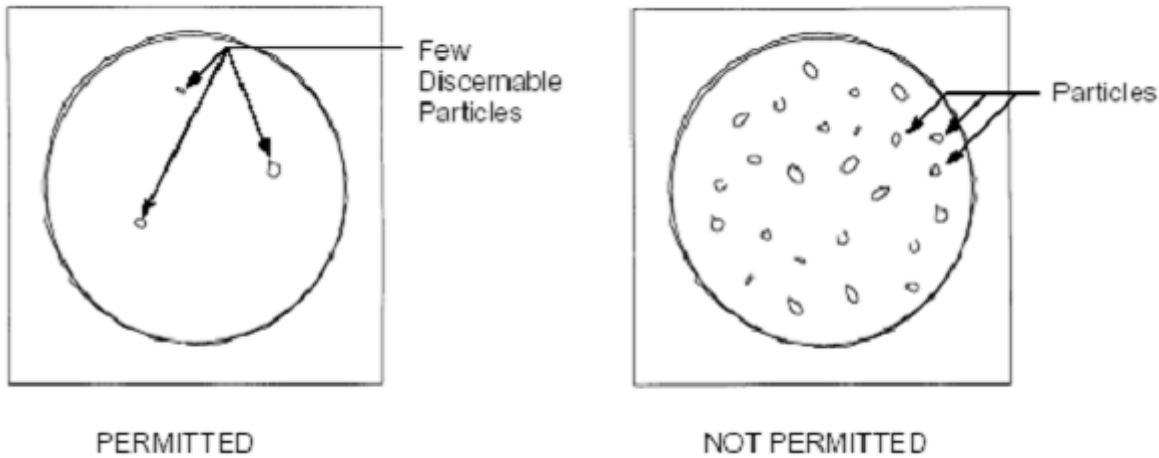
Figure 16. Particle Contamination of the Endface of an Optical Fiber
