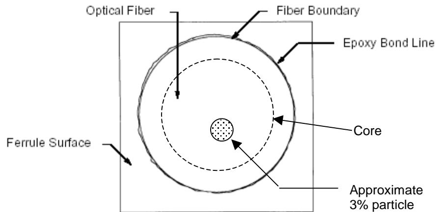
Figure 15. Typical Endface of an Optical Fiber
