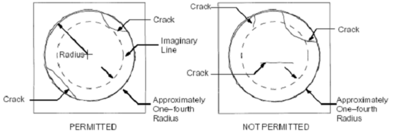
Figure 19. Cracks on the Endface of an Optical Fiber
