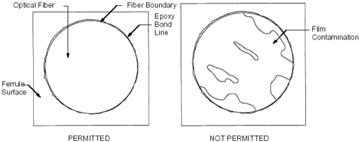
Figure 17. Film Contamination of the Endface of an Optical Fiber
