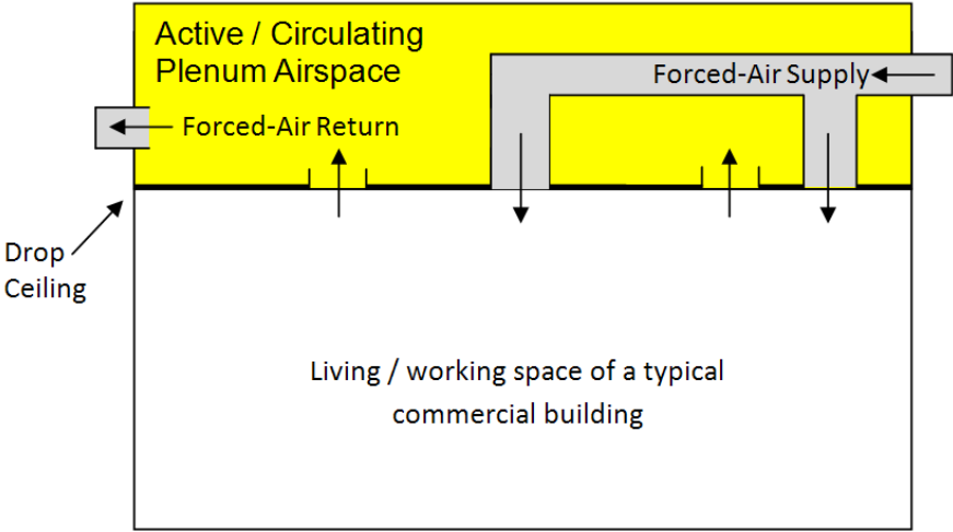
Figure 1. Building With a Plenum Airspace
