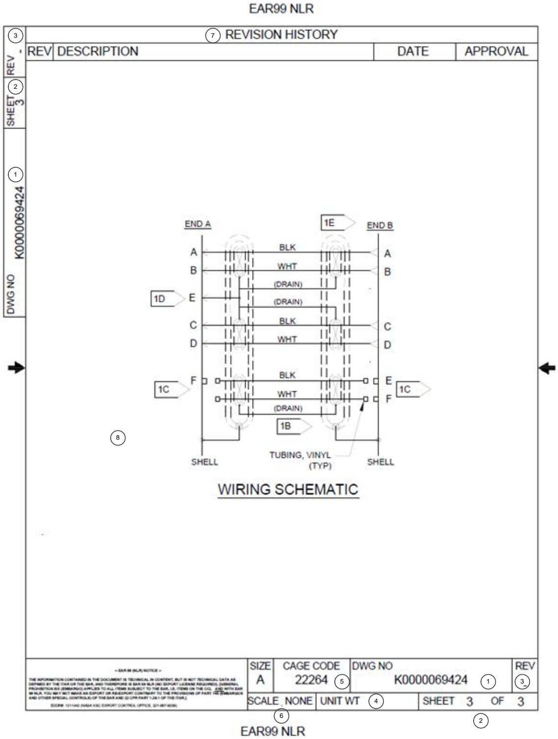
Figure 14. Cable Subassembly Drawing – Continuous/Last Page
