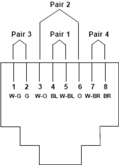
Figure 6. Recommended Eight-Position Jack Pin/Pair Assignments (T568A)
