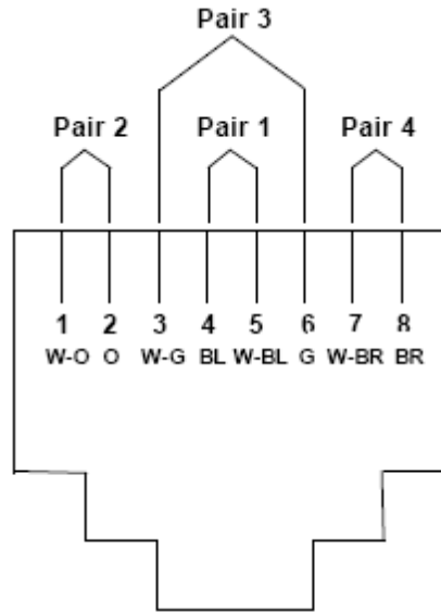
Figure 7. Optional Eight-Position Jack Pin/Pair Assignment (T568B)
