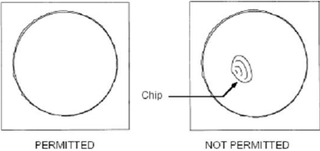
Figure 20. Example of a Chip on the Endface of an Optical Fiber
