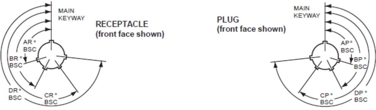
Figure 9. 38999 Polarization Angles
