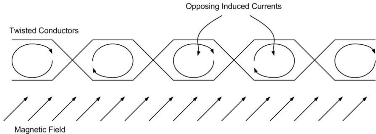
Figure 4. Twisted Conductor
