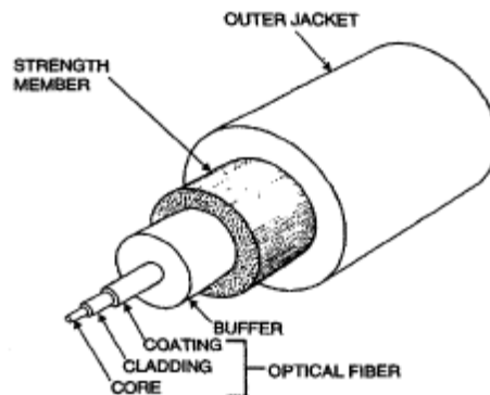
Figure 8. Parts of a Typical Fiber-Optical Cable
