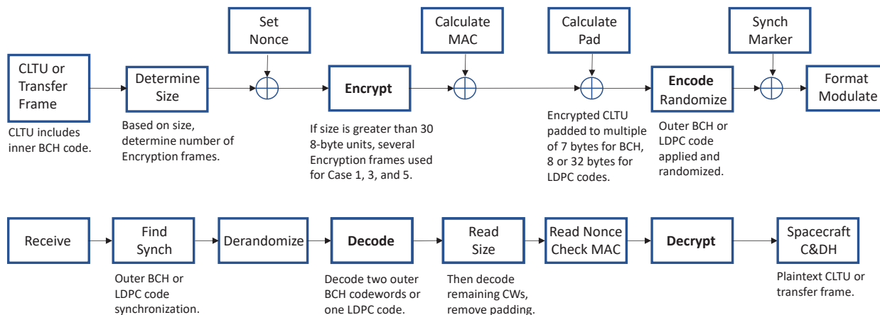
Figure 6. Function Flow for Security and Coding
