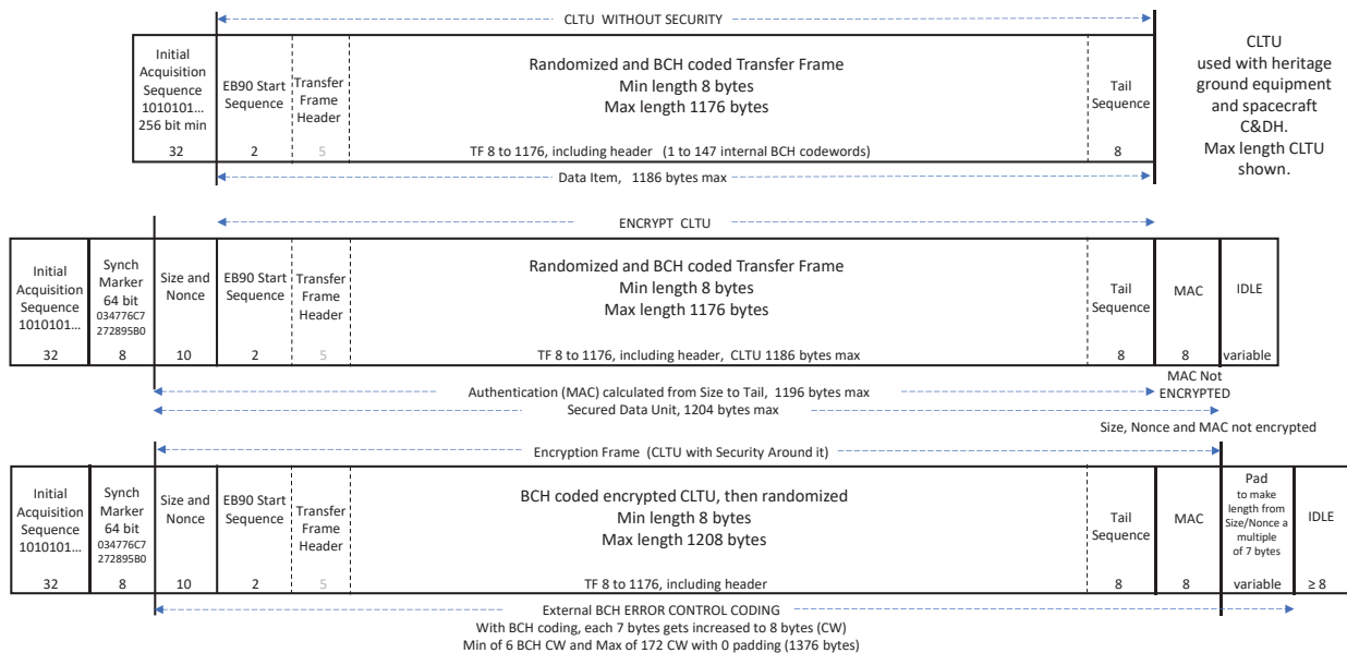
Figure 9. Use Case 2: CLTU Max Length Transfer Frame in single Encryption Frame
