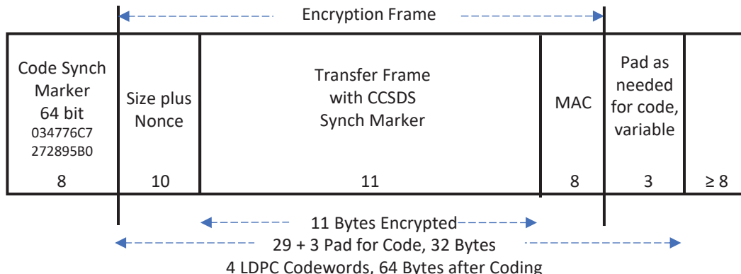
Figure 13. Use Cases 5 and 6: Transfer Frame - Minimum Length, LDPC Coded
