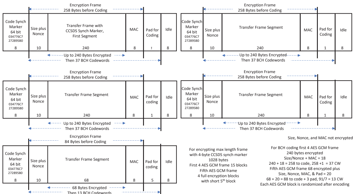
Figure 11. Use Case 3: Transfer Frame Max Length in 5 Encryption Frames, BCH Coded
