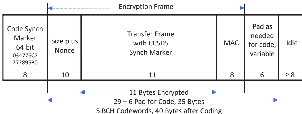
Figure 10. Use Cases 3 and 4: Transfer Frame Minimum Length – BCH Coded
