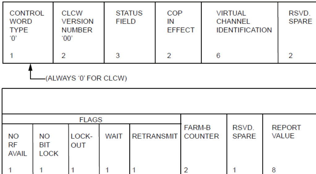
Figure 4-6: Communications Link Control Word
