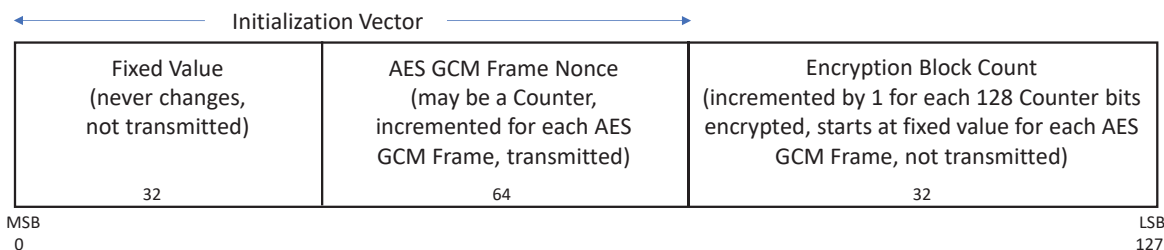
Figure 3. Example Counter Block
