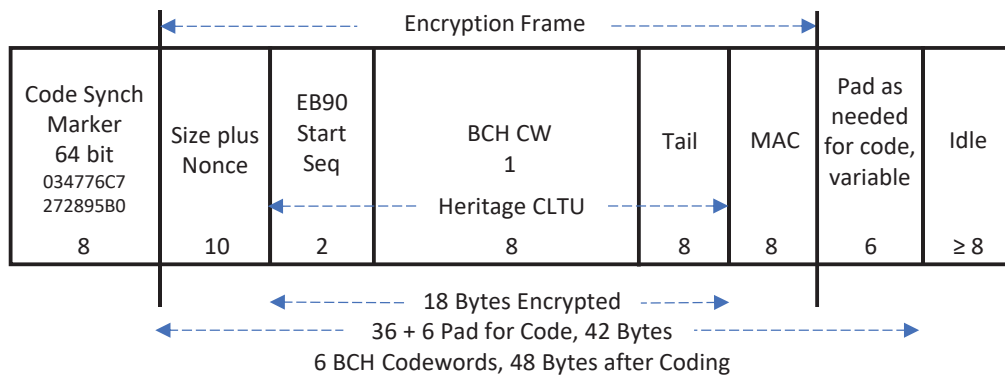
Figure 7. Use Cases 1 and 2: HCLTU with Min Length Transfer
