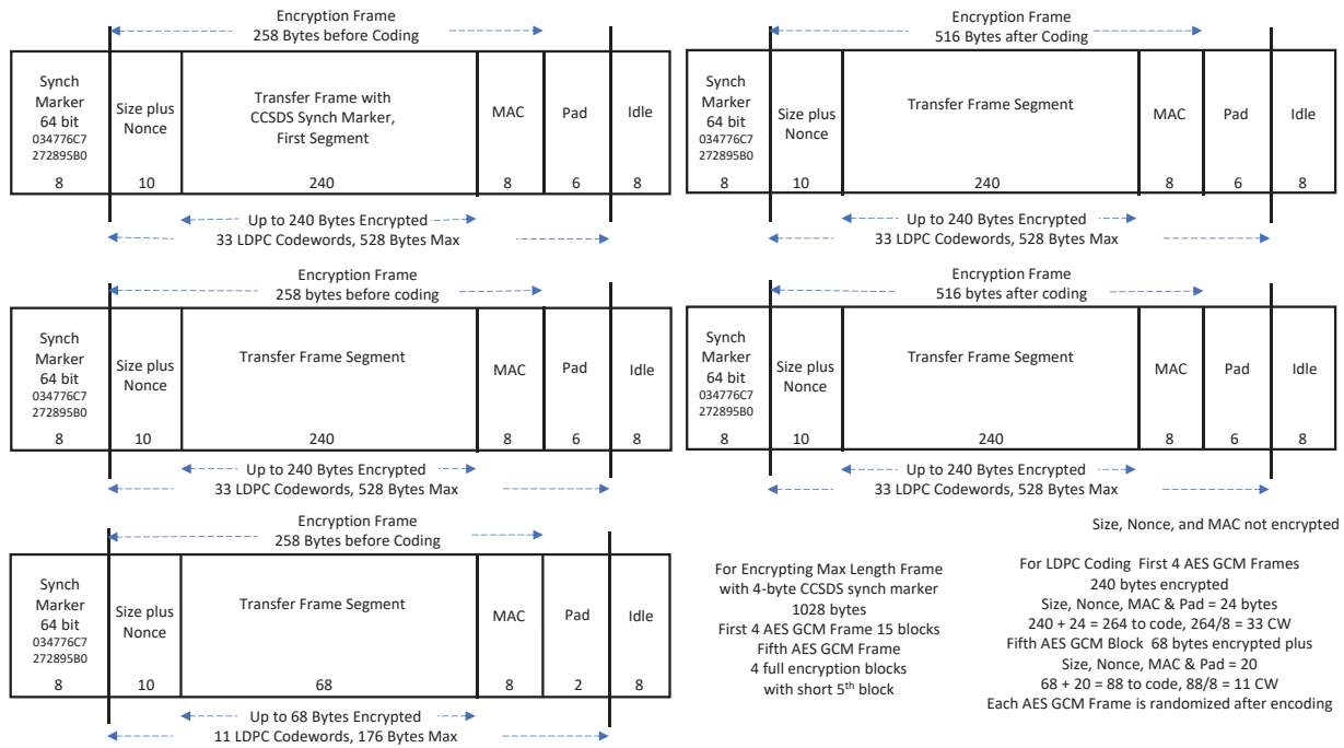
Figure 14. Use Case 5: Transfer Frame Maximum Length in 5 Small Encryption Frames, LDPC Coded
