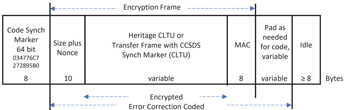
Figure 1. Bulk Secured and Coded Data
