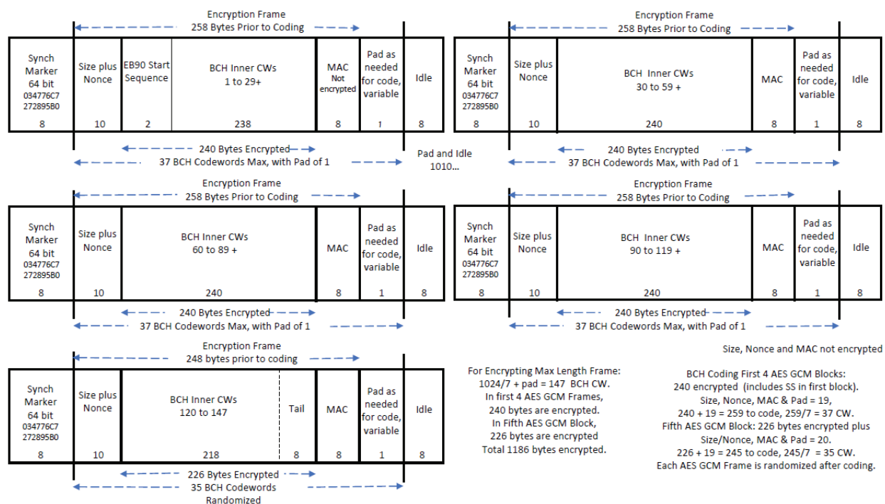
Figure 8. Use Case 1: HCLTU Max Length Transfer Frame in 5 Small Frames
