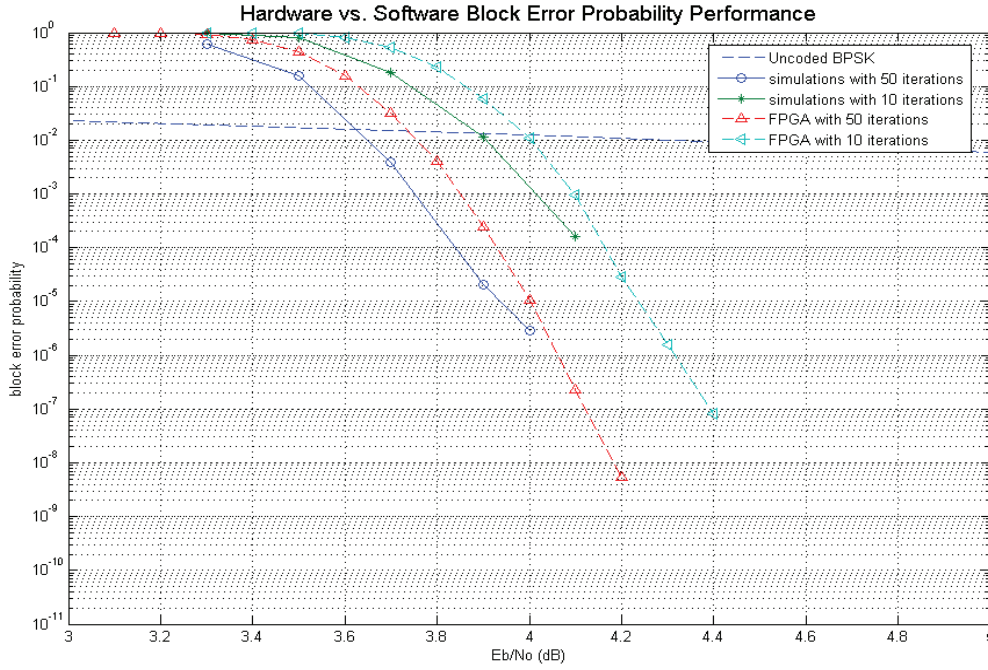
Figure 10. Block Error Rate Test Results
