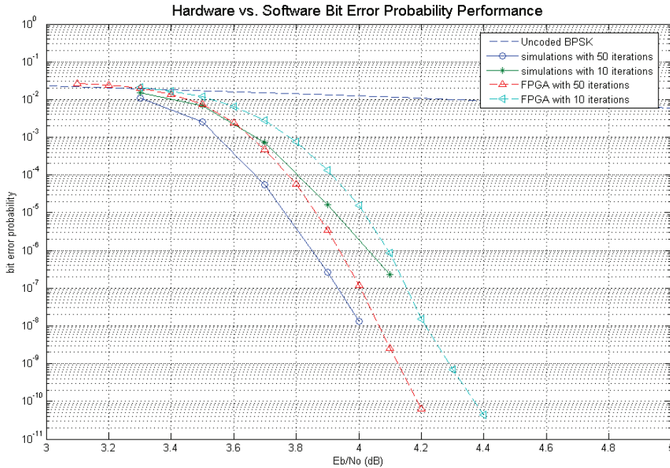
Figure 9. Bit Error Rate Test Results
