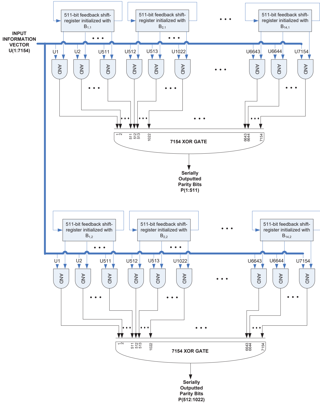
Figure 7. Encoder Diagram
